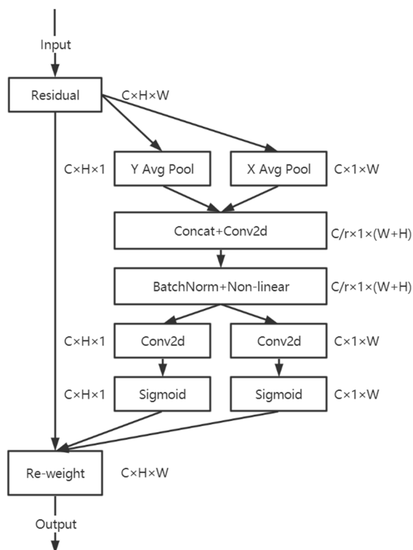
FIGURE 3. CoordAttention structure.
