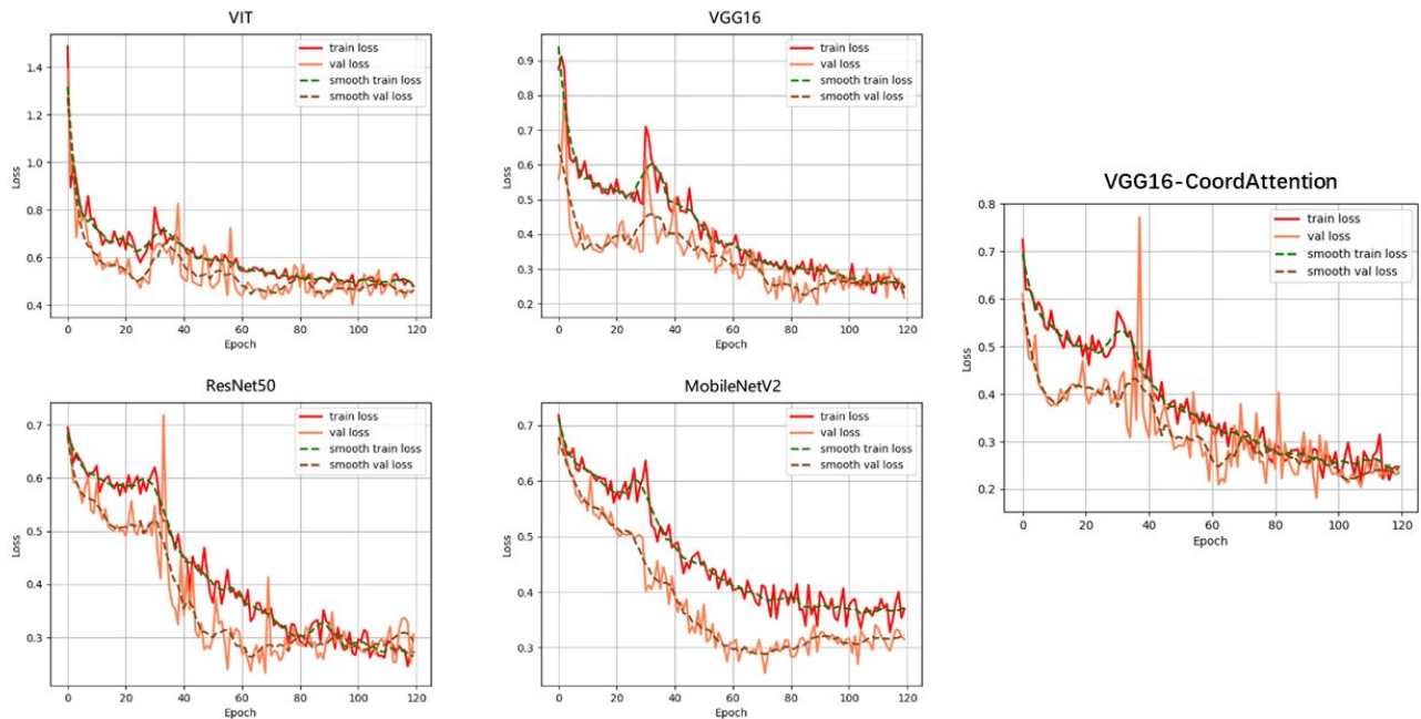
FIGURE 5. The loss curves of the training set and the validation set of the five backbone networks are frozen on the Shenzhen dataset (Red represents train loss, yellow represents val loss, green represents smooth train loss, and brown represents smooth val loss).
