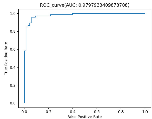
FIGURE 6. ROC curve on test set.
